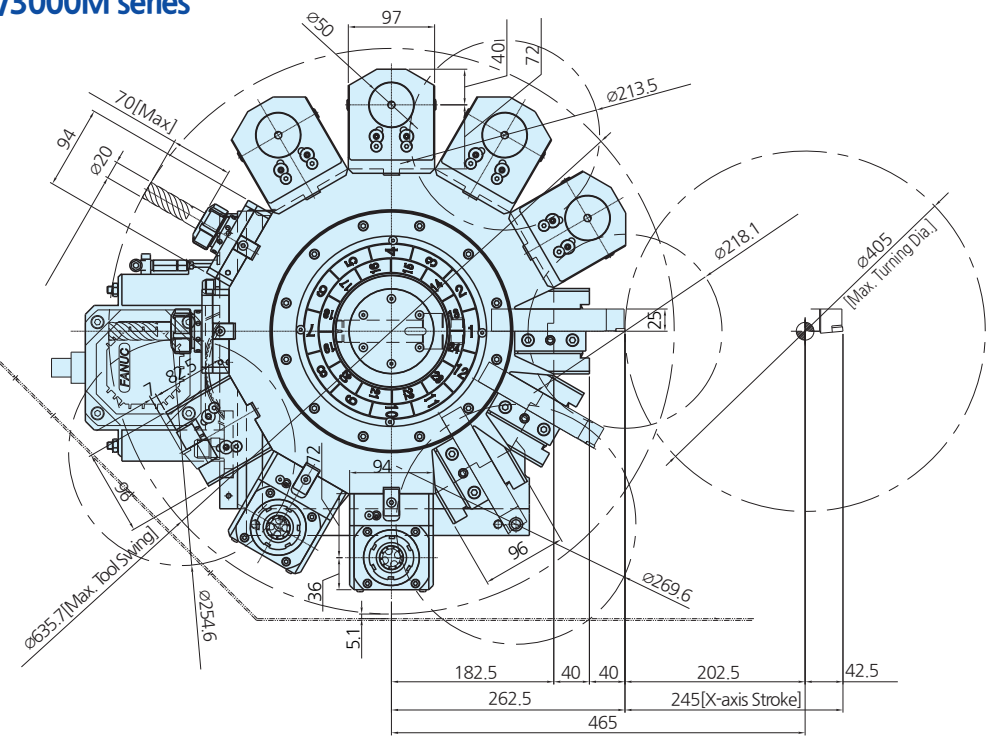
SL 2500M/3000M series
