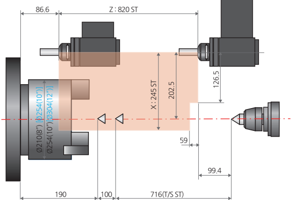
Angular milling head
