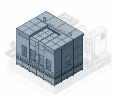
Full Splash Guard (With Roof)
